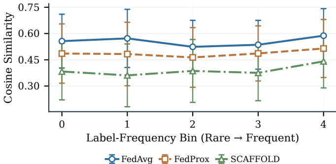
Attention Alignment by Label Frequency
